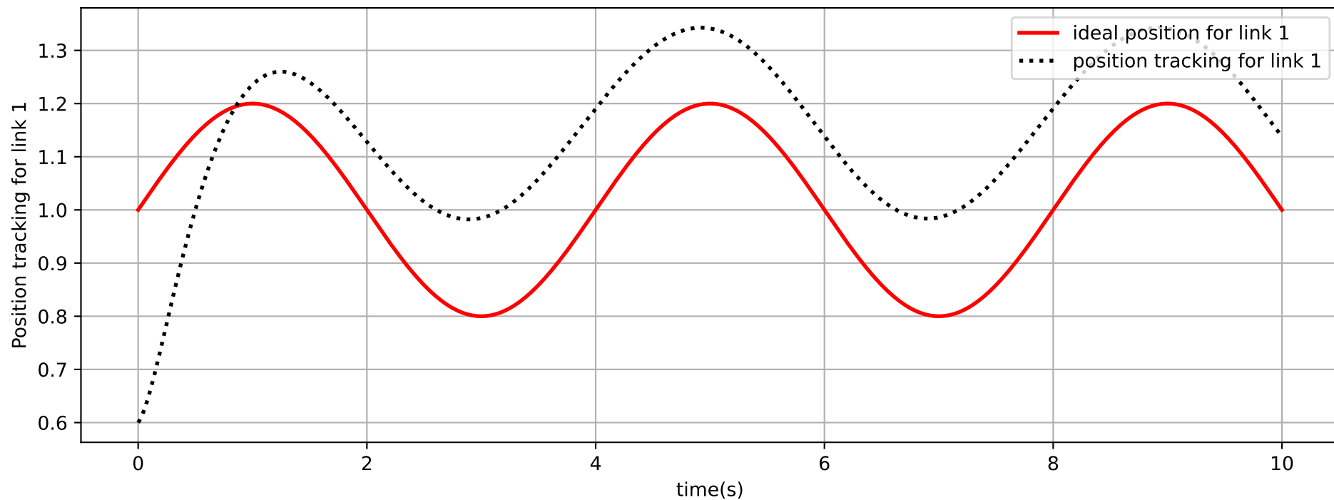
Position Tracking Performance ( S=1 , S1=1 , m=5 )
